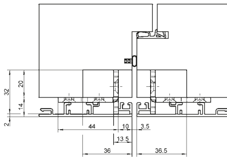
timber/aluminium system
